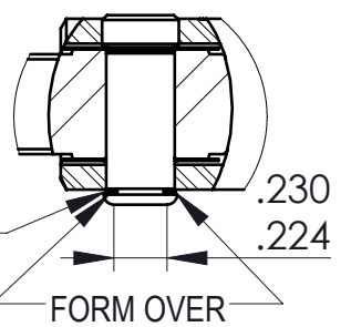
DETAIL A SCALE 1.5 : 1 DEFORM BEFORE CALIBRATION
