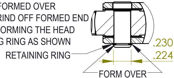
DETAIL A SCALE 2 : 1.5 DEFORM BEFORE CALIBRATION
