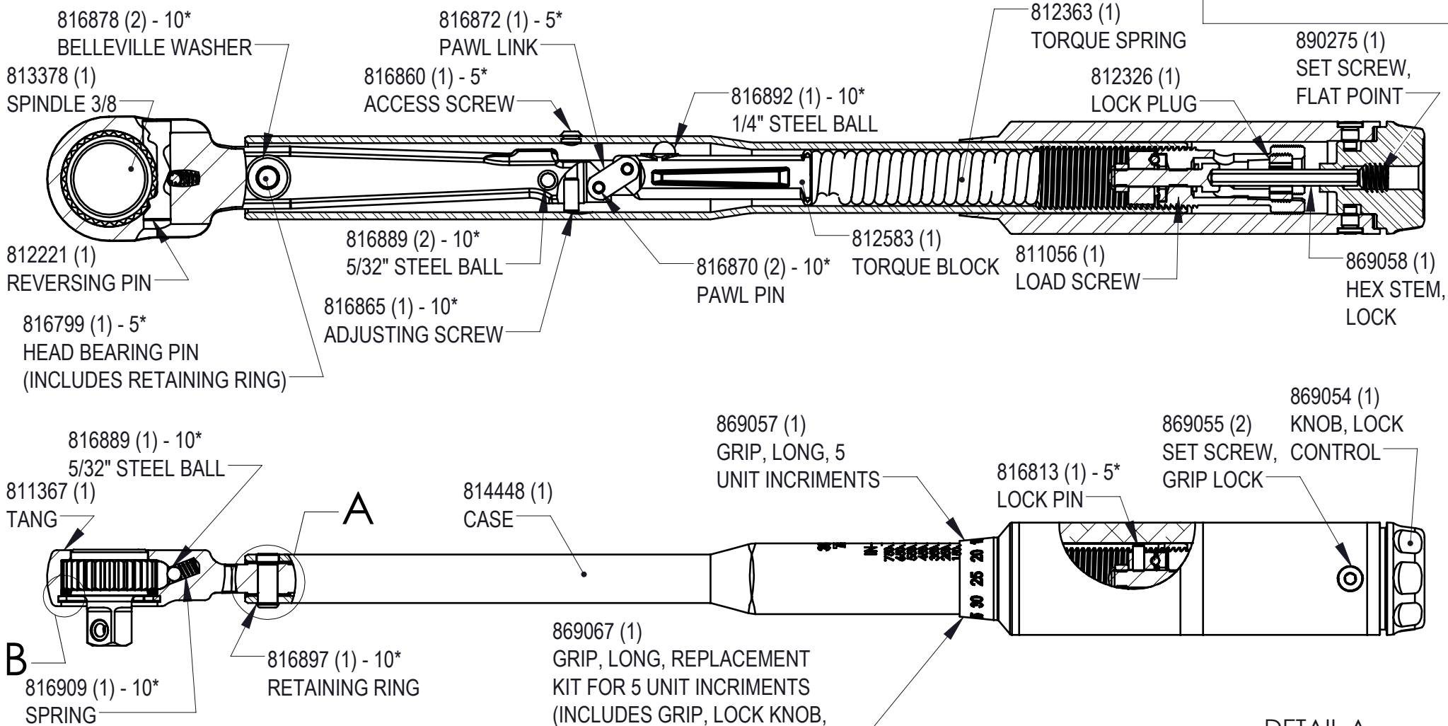
DETAIL A SCALE 2 : 1.5 DEFORM BEFORE CALIBRATION
