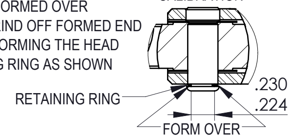
DETAIL A SCALE 1.5 : 1 DEFORM BEFORE CALIBRATION
